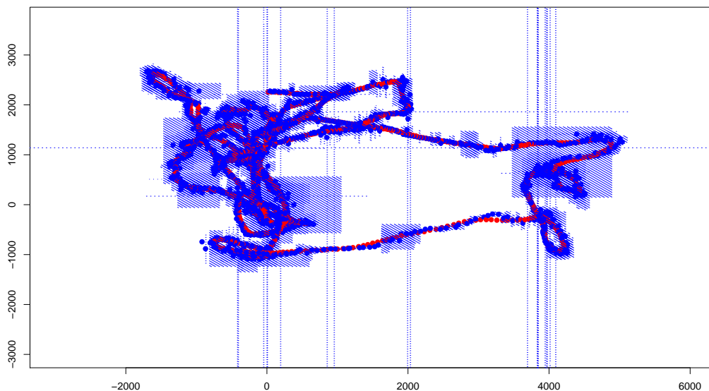
Figure 4.5: Blue dot: 5-step-ahead predicted position; blue square: 95%-prediction rectangle; red dot: true recorded position. The horizontal and vertical lines are artefacts of the algorithm.
