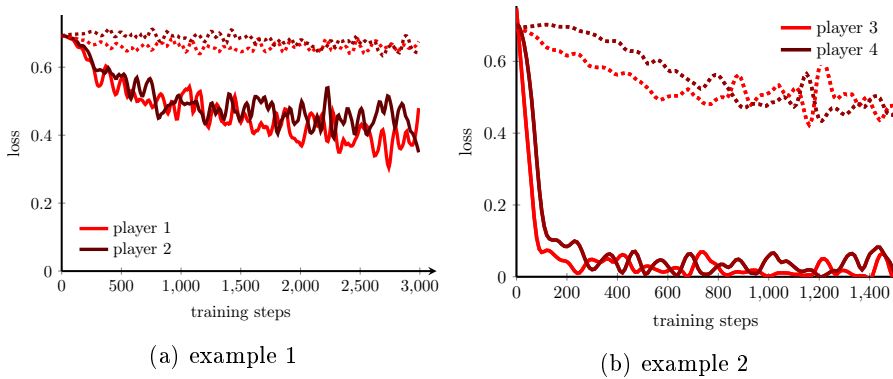
Figure 4.12: Two examples of the Discriminator loss function for both players as a function of the number of training steps. The solid lines are the results for uncentered data and the dashed lines contain the results for the centered data. The two examples contain four different players.
