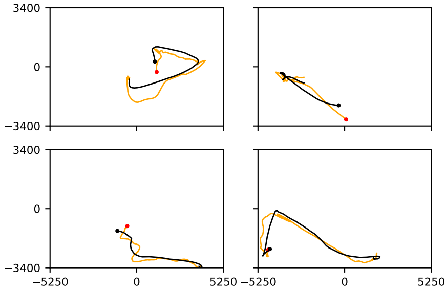
Figure 4.10: A collection of sampled trajectories (orange) and an approximation calculated by the VAE (black). In general, the approximating trajectories are much smoother. We chose \sigma_X \approx 0.15 in training the VAE.
