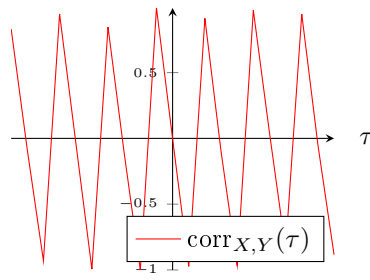
Figure 1.7: Correlation of Y and X
