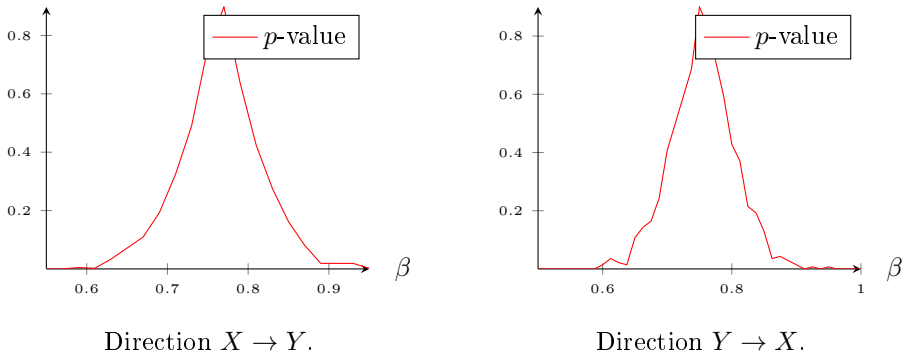
Figure 1.8: Reliability of the linear description as function of \beta .
