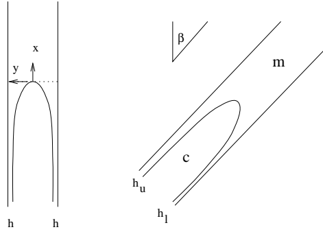
Figure 2: Steady interface between displacer c and displaced fluid m ; symmetric and non-symmetric front.
